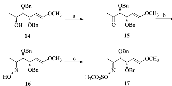
Scheme 5. Reagents and conditions: a) PDC, CH 3 CN, 4-Å molecular sieves, room temp. (95%); b) NH 2 OH·HCl, NEt 3 , EtOH/THF 1:1, 40 °C (80%); c) CH 3 SO 2 Cl, NEt 3 , CH 2 Cl 2 , room temp. (90%)
