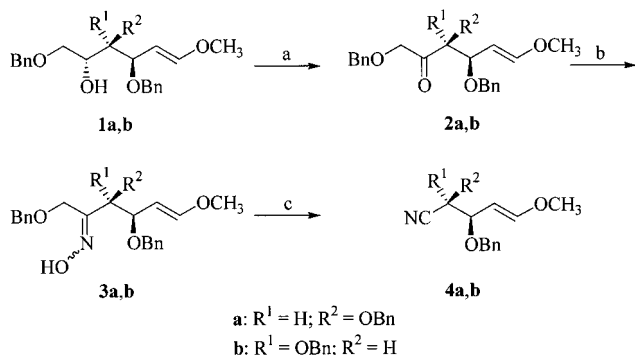
Scheme 1. Reagents and conditions: a) PDC, CH 3 CN, 4-Å molecular sieves, room temp. (90–95%); b) NH 2 OH·HCl, NEt 3 , EtOH/THF 1:1, 40 °C, (75–80%); c) CH 3 SO 2 Cl, NEt 3 , CH 2 Cl 2 , room temp. (60–70%)
