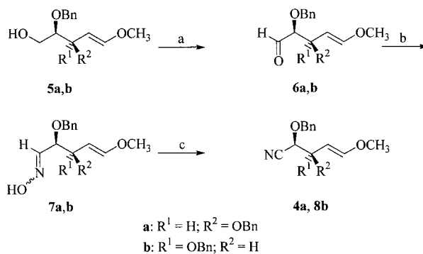
Scheme 2. Reagents and conditions: a) PDC, CH 3 CN, 4-Å molecular sieves, room temp. (80%); b) NH 2 OH·HCl, NEt 3 , EtOH/THF 1:1, 40 °C, (90%); c) CH 3 SO 2 Cl, NEt 3 , CH 2 Cl 2 , room temp. (90%)
