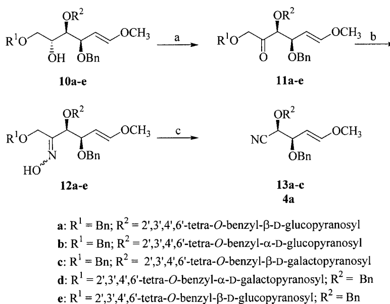
Scheme 4. Reagents and conditions: a) PDC, CH 3 CN, 4-Å molecular sieves, room temp. (90–95%); b) NH 2 OH·HCl, NEt 3 , EtOH/THF 1:1, 40 °C (75–80%); c) CH 3 SO 2 Cl, NEt 3 , CH 2 Cl 2 , room temp. (30–70%)
