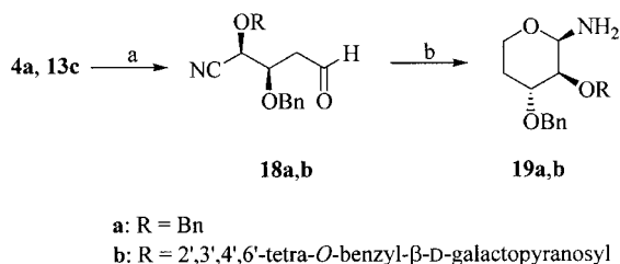
Scheme 6. Reagents and conditions: a) THF/4 N HCl (5:1), room temp.; b) NaBH 4 , THF/EtOH (1:1), reflux
